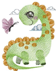
Ape3038a_001.vip 2.98x3.83 inches; 6,775 stitches 11 thread changes; 8 colors
