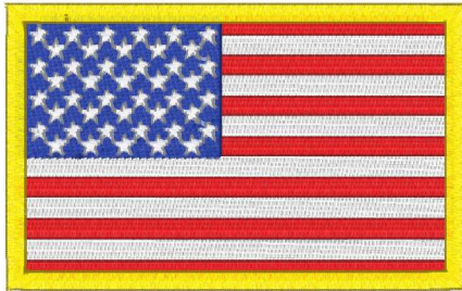
Flag Usa 07102022 4 Inch.vip 3.80x2.38 inches; 18,203 stitches 5 thread changes; 4 colors
