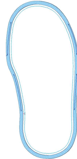
Ewc226_rightmediumsole.vip 4.57x9.90 inches; 5,338 stitches 6 thread changes; 5 colors
