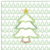
Block 6.vip
