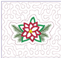
Block 1.vip
