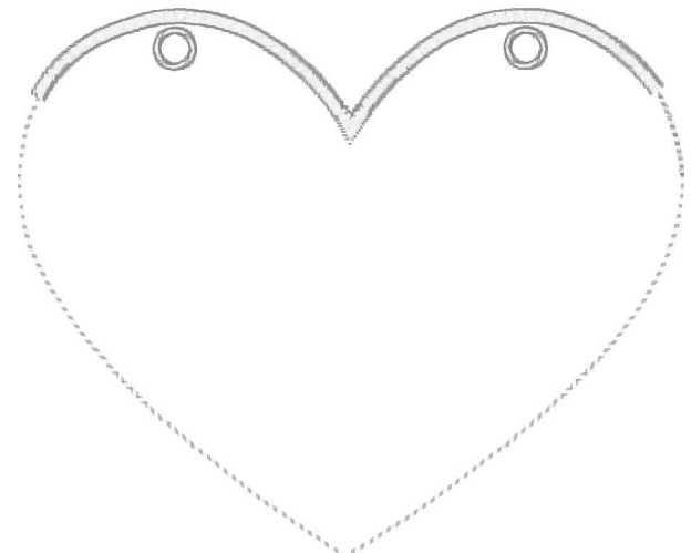
Heart Bag 6a.vip 4.93x4.07 inches; 1,407 stitches 3 thread changes; 2 colors
