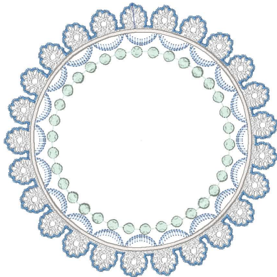
Oae044_scollop_doily3.vip 7.80x7.82 inches; 31,859 stitches 9 thread changes; 9 colors
